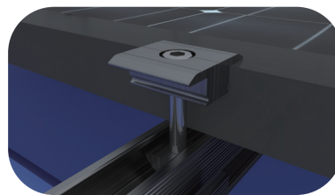
Inter Clamp Fixing
