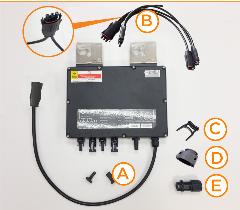
APSYSTEMS YC600
