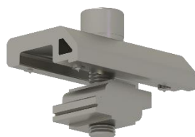
Rail Clamp for T-Rail with grounding/earthing pins Part No.: ER-RC-T/G
