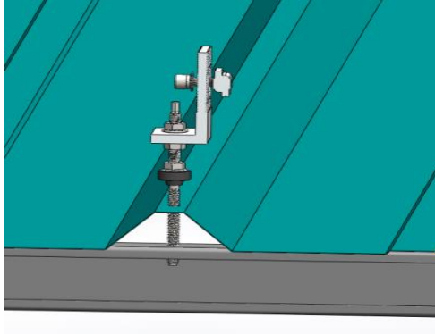
Assembly view : Hanger Bolt & L-foot
